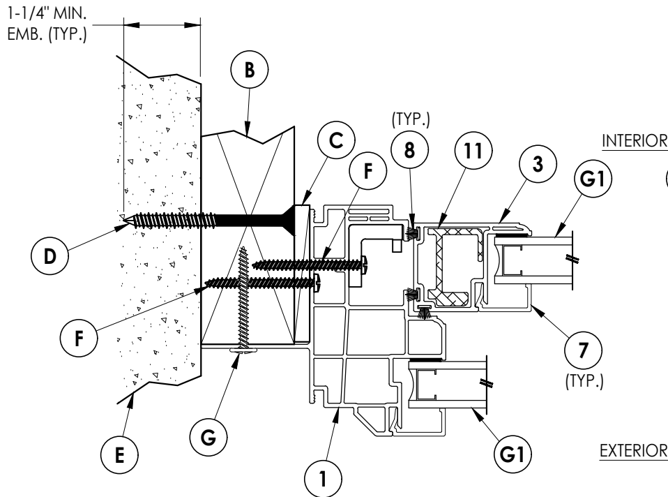
1 2 HORIZONTAL CROSS SECTION Shown w/ 2X Buck
