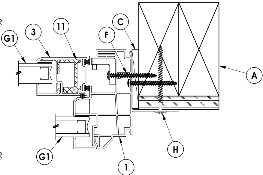
2 2 HORIZONTAL CROSS SECTION Shown w/ 2X Stud Construction
