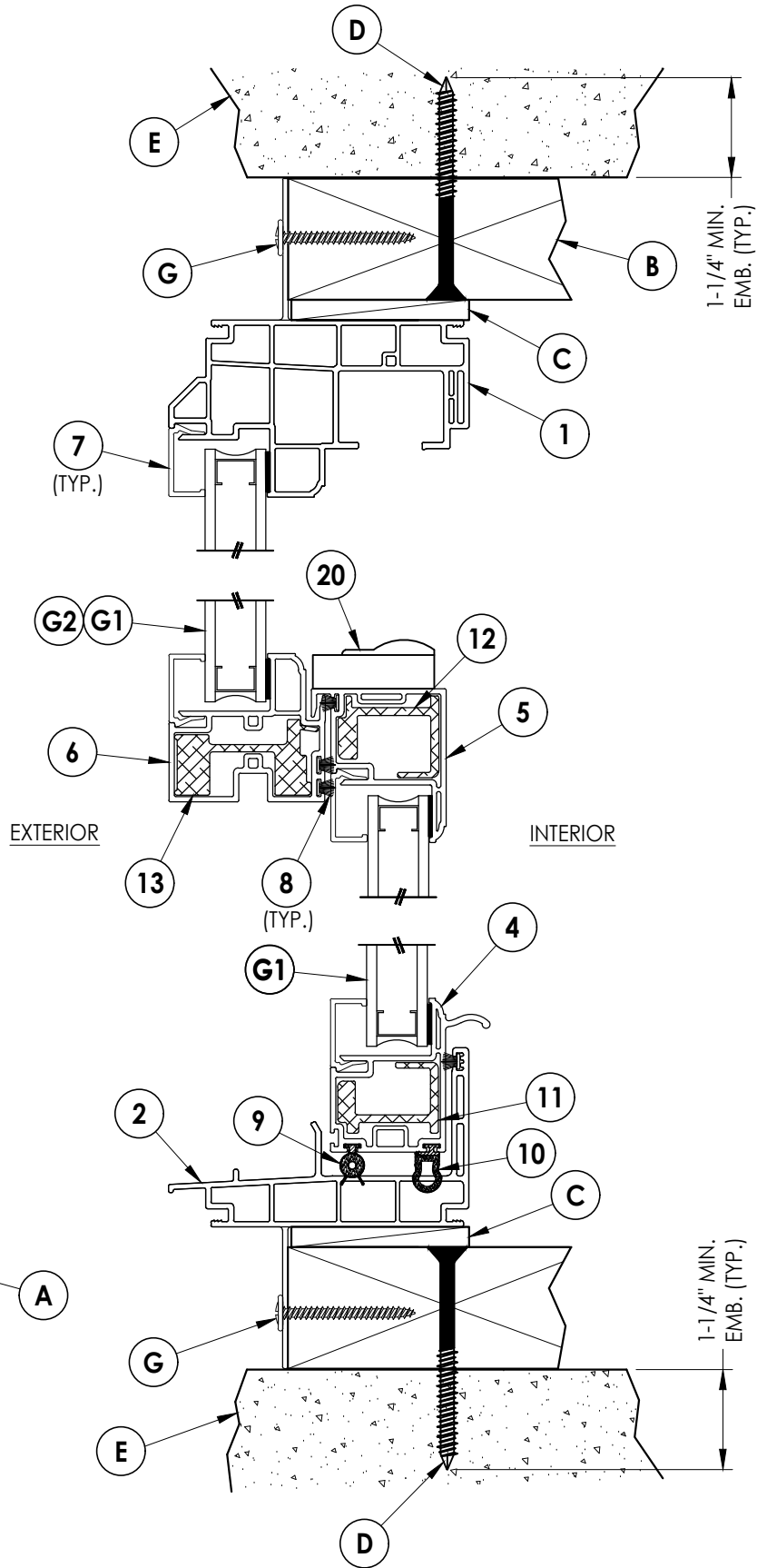
3 2 HORIZONTAL CROSS SECTION Shown w/ 2X buck
